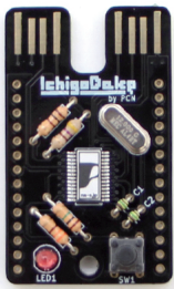
JavaScript
